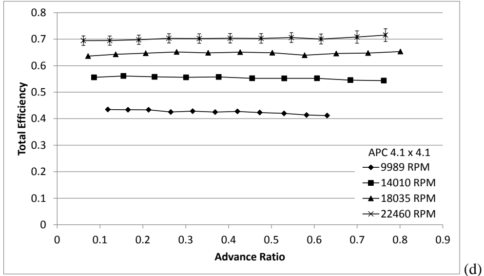
Figure 78: APC 4.1 x 4.1 Dynamic Test Results: (a) Coefficient of Thrust, (b) Coefficient of Power, (c) Propeller Efficiency, (d) Total Efficiency.
