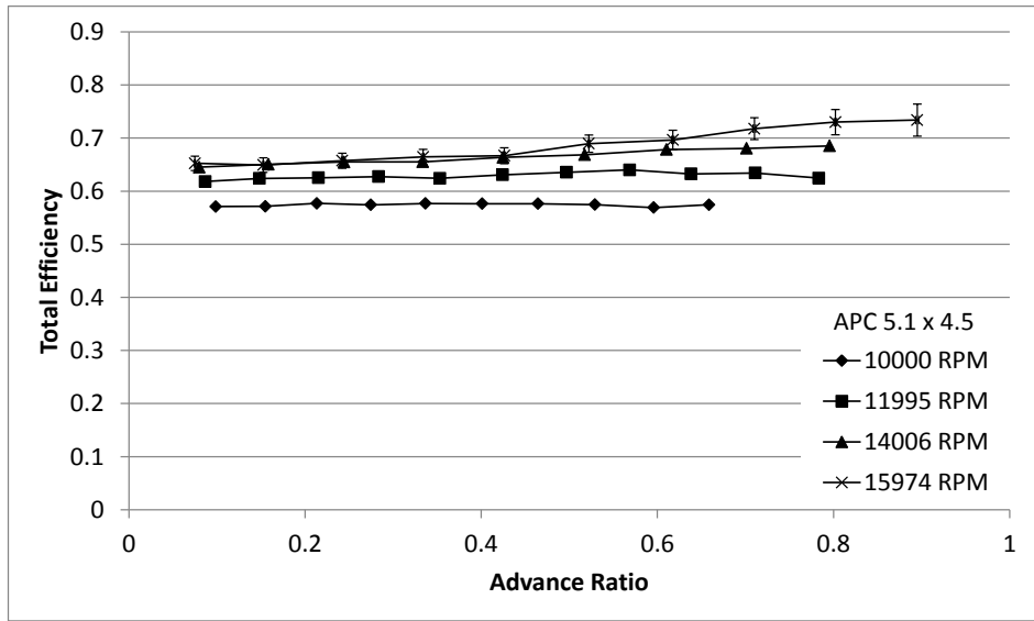
Figure 86: APC 5.1 x 4.5 Dynamic Test Results: (a) Coefficient of Thrust, (b) Coefficient of Power, (c) Propeller Efficiency, (d) Total Efficiency.
