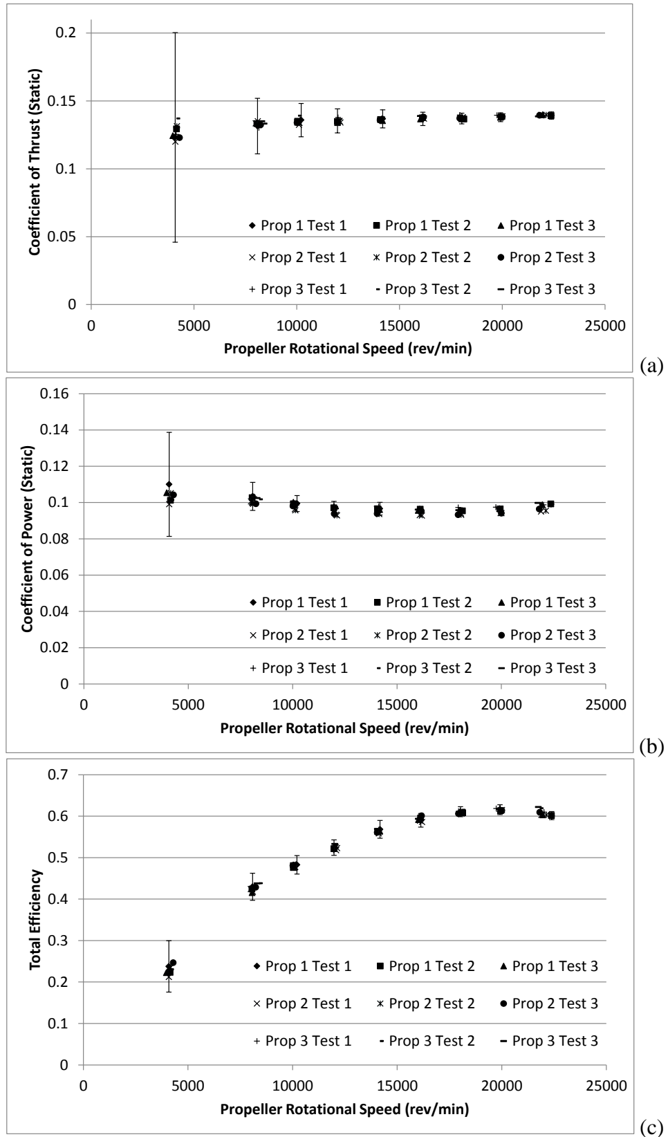
Figure 4: Comparison of Three Identical Propellers (Graupner 4.7 \times 4.7 ): (a) Static Coefficient of Thrust, (b) Static Coefficient of Power, (c) Static Total Efficiency.
