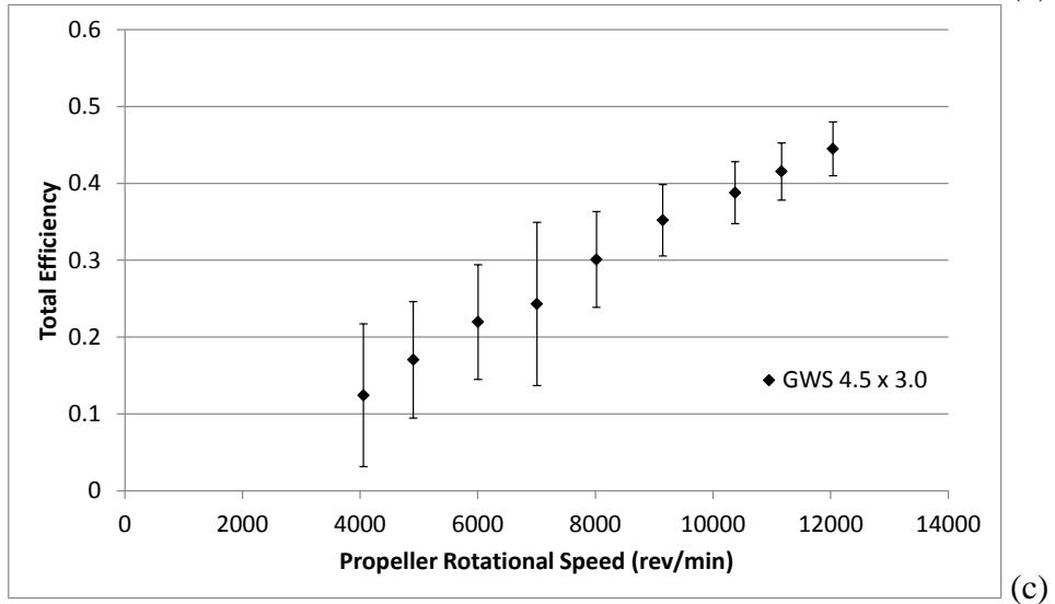
Figure 72: GWS 4.5 x 3.0 Static Test Results: (a) Coefficient of Thrust, (b) Coefficient of Power, (c) Total Efficiency.
