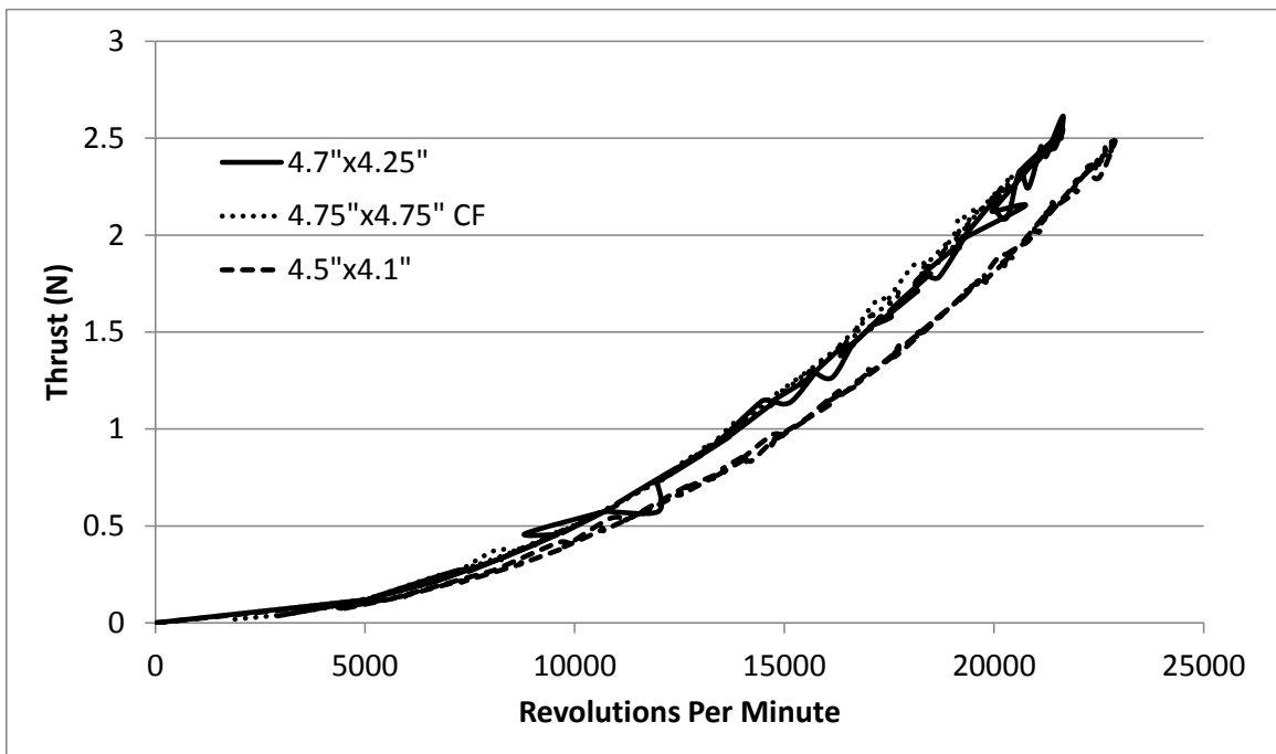
Figure 39: Stepped Throttle Thrust versus RPM for Various Propellers
