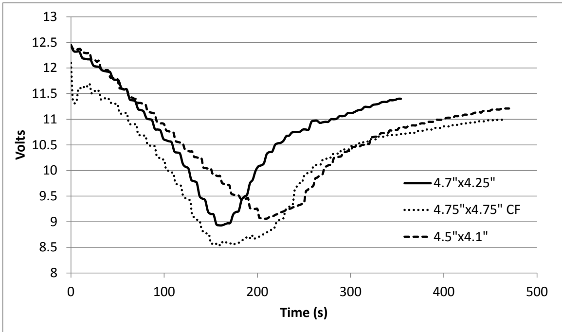
Figure 38: Stepped Throttle Voltage versus Time for Various Propellers
