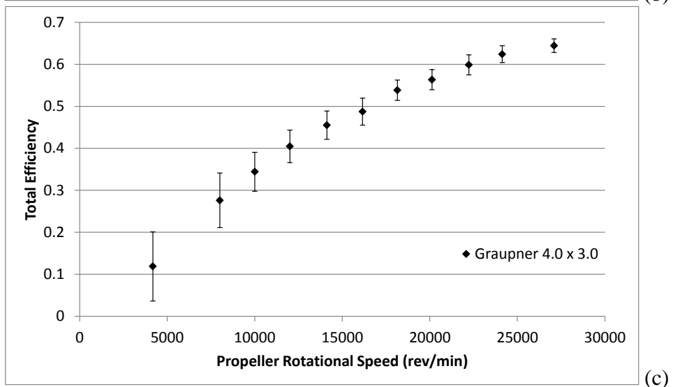
Figure 57: Graupner 4.0 x 3.0 Static Test Results: (a) Coefficient of Thrust, (b) Coefficient of Power, (c) Total Efficiency.
