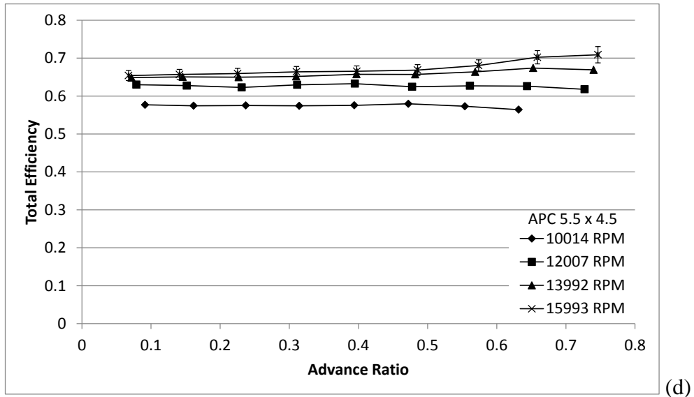
Figure 89: APC 5.5 x 4.5 Dynamic Test Results: (a) Coefficient of Thrust, (b) Coefficient of Power, (c) Propeller Efficiency, (d) Total Efficiency.
