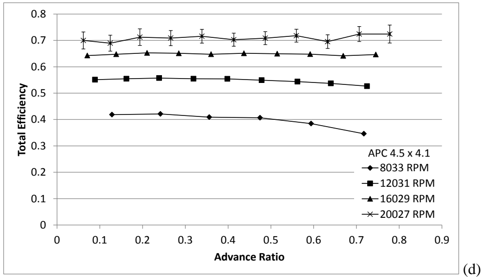
Figure 81: APC 4.5 x 4.1 Dynamic Test Results: (a) Coefficient of Thrust, (b) Coefficient of Power, (c) Propeller Efficiency, (d) Total Efficiency.
