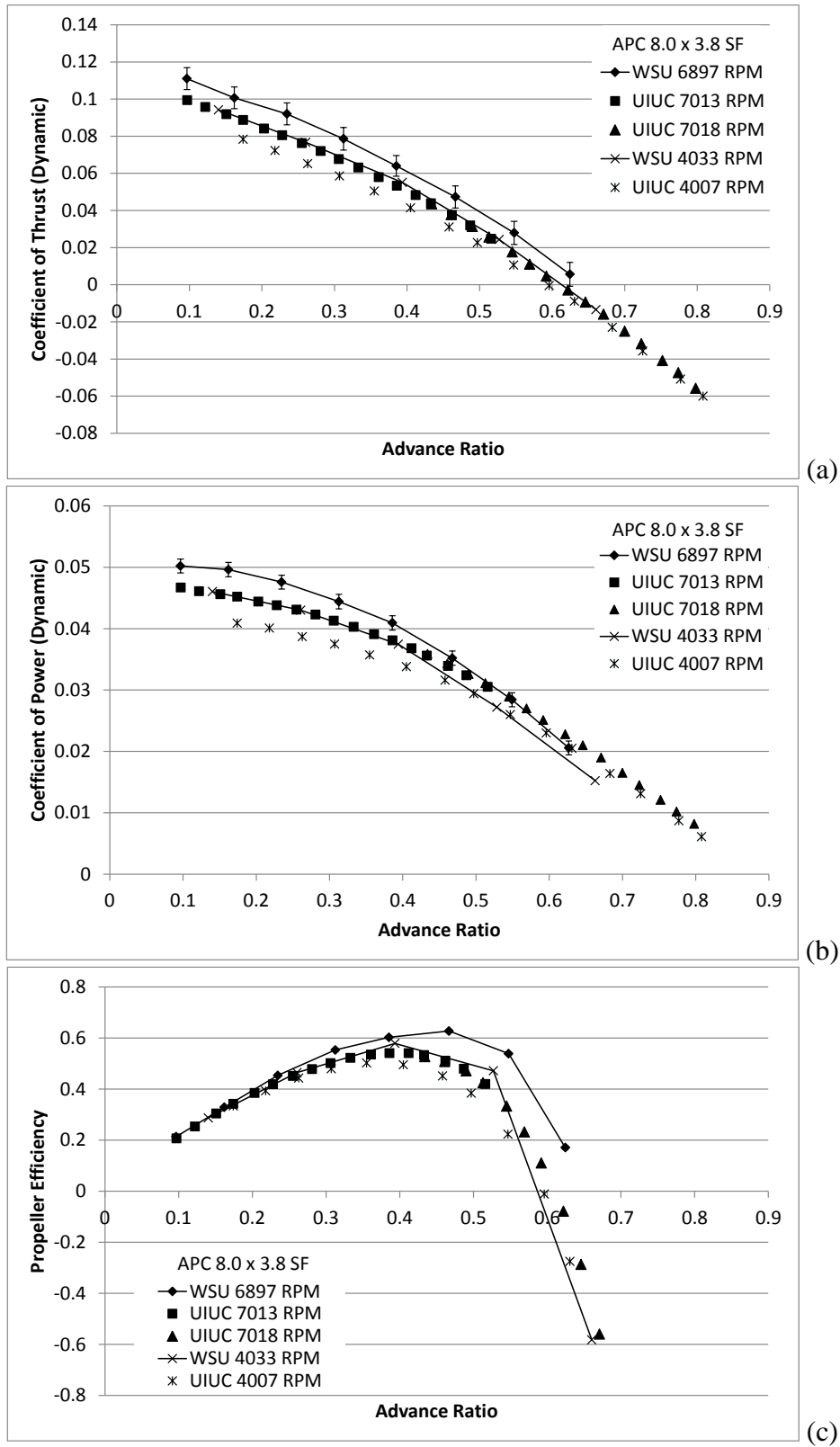
Figure 9: Comparison of Present Results to Selig (2012) (APC 8.0 \times 3.8 SF): (a) Dynamic Coefficient of Thrust, (b) Dynamic Coefficient of Power, (c) Propeller Efficiency.
