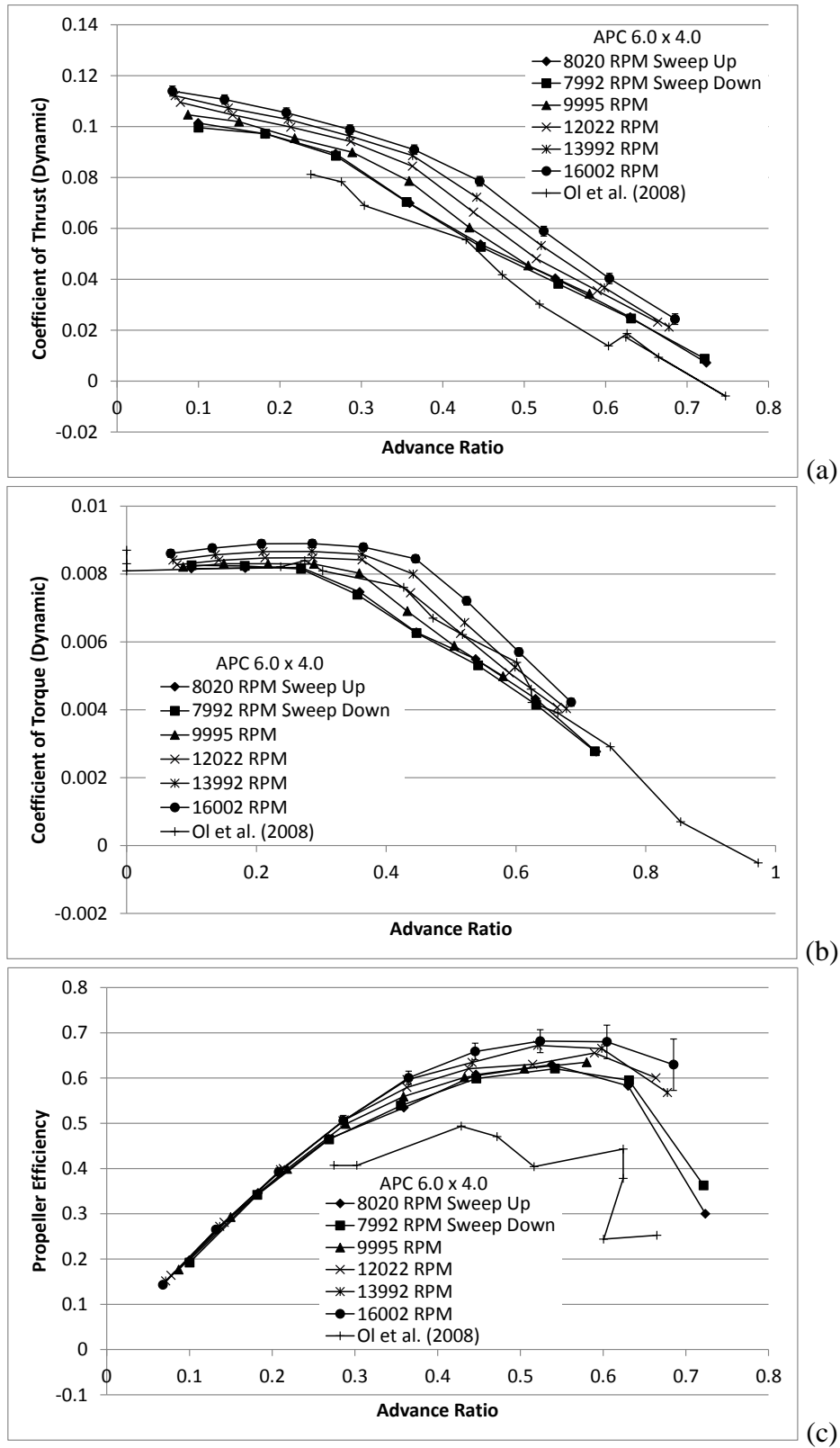
Figure 10: Comparison of Present Results to Ol et al. (2008) (APC 6.0 × 4.0): (a) Dynamic Coefficient of Thrust, (b) Dynamic Coefficient of Torque, (c) Propeller Efficiency.
