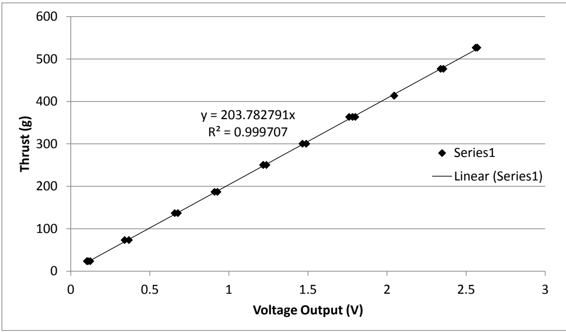
Figure 21: Calibration Equation of Load Cell
