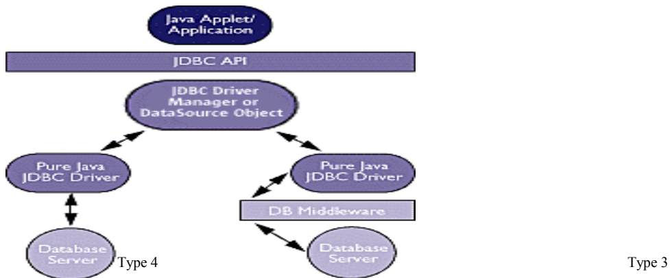
Figure 11: DATABASES VIA THE PURE JAVA JDBC TECHNOLOGY-BASED DRIVERS.
