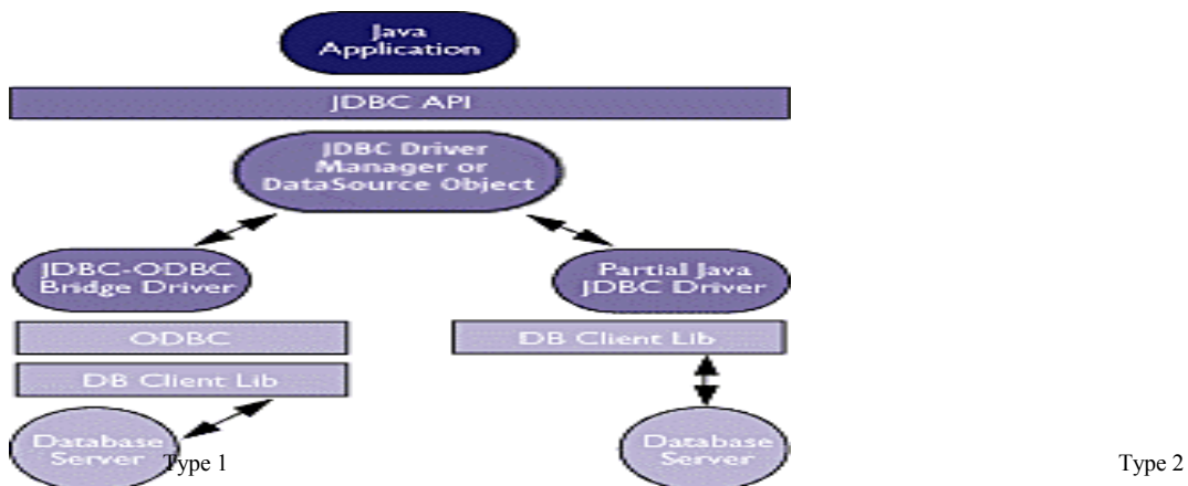
Figure 12: JDBC connectivity using ODBC drivers and existing database client libraries.
