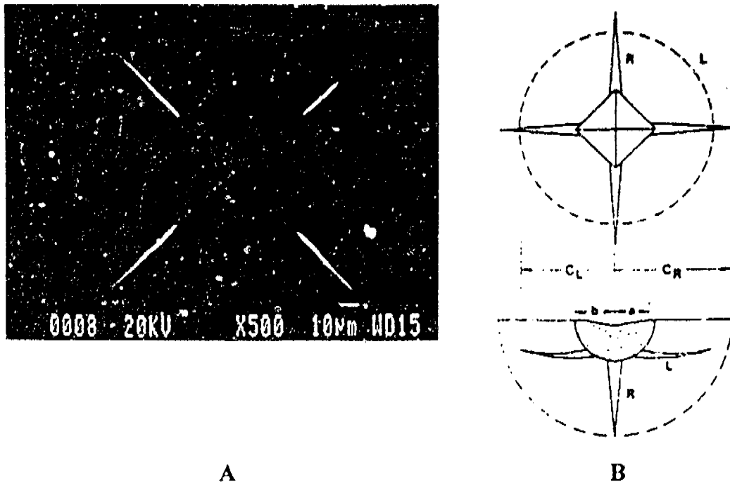
Figure 3. SEM photograph of a Vickers indentation on a zirconia orthodontic bracket (A) (Tilson, 1994; (B) top and side-view diagrams of an ideal indentation pattern, where a + b represents the diagonal length and C_L and C_R represent the left and right crack lengths (Morena et al. , 1986).
