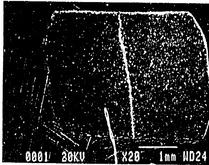
Figure 17. SEM photograph of the stress-concentrating defect in the base of the Clarity bracket (low magnification).
