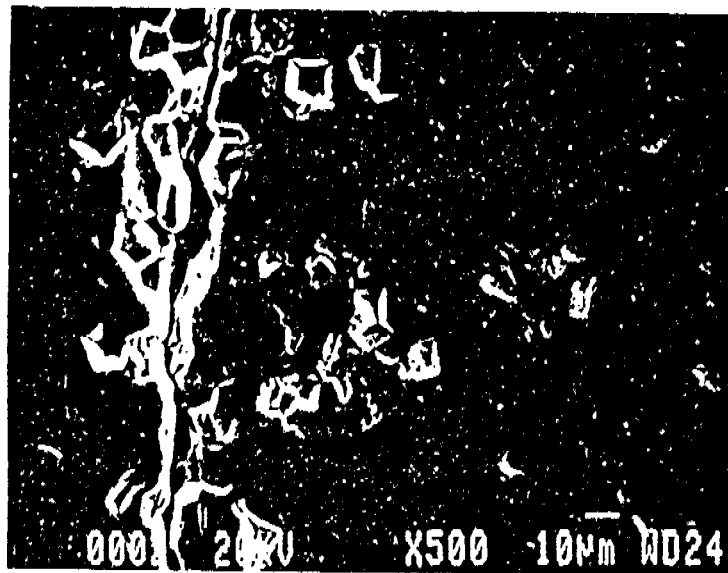
Figure 18. SEM photograph of the stress-concentrating defect in the base of the Clarity bracket (high magnification).
