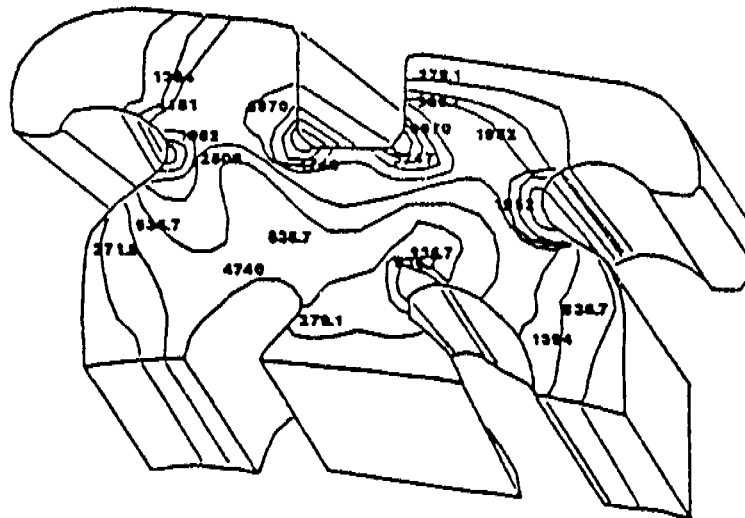
Figure 4. Finite element analysis showing stress distribution in a bracket subjected to loading (Swartz, 1988).
