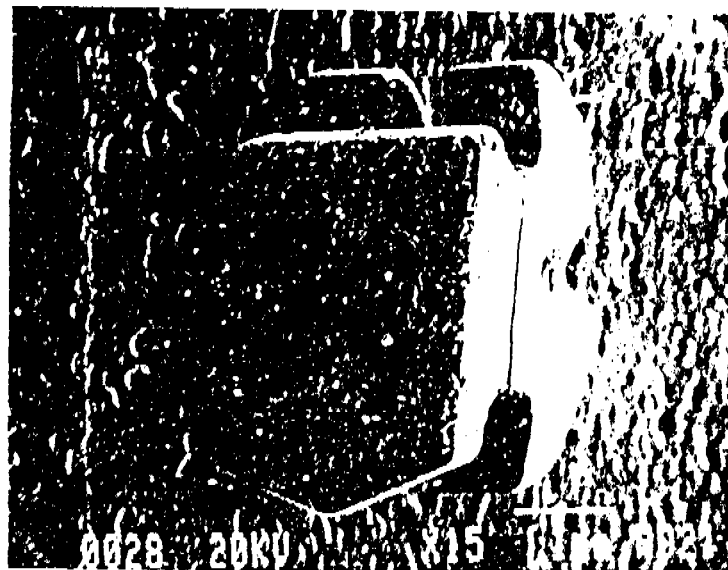
Figure 20. The Contour bracket base employs protruding crystals for mechanical retention.
