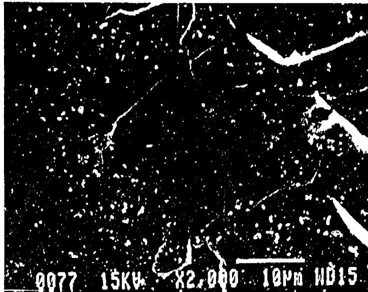
Figure 7. A 1 kg indentation on the polished base of an Allure bracket.
