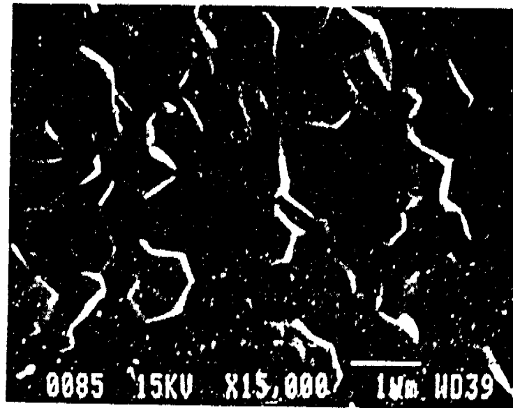
Figure 15. SEM photograph of the fracture surface of a Contour bracket.
