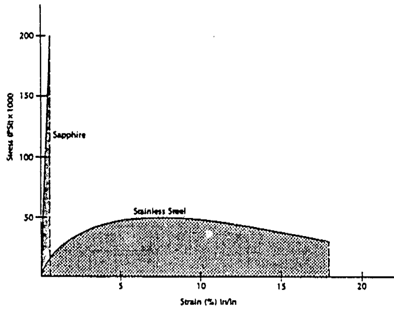
Figure 1. Stress-strain curves for sapphire (single-crystal aluminum oxide) and stainless steel (Scott, 1988).
