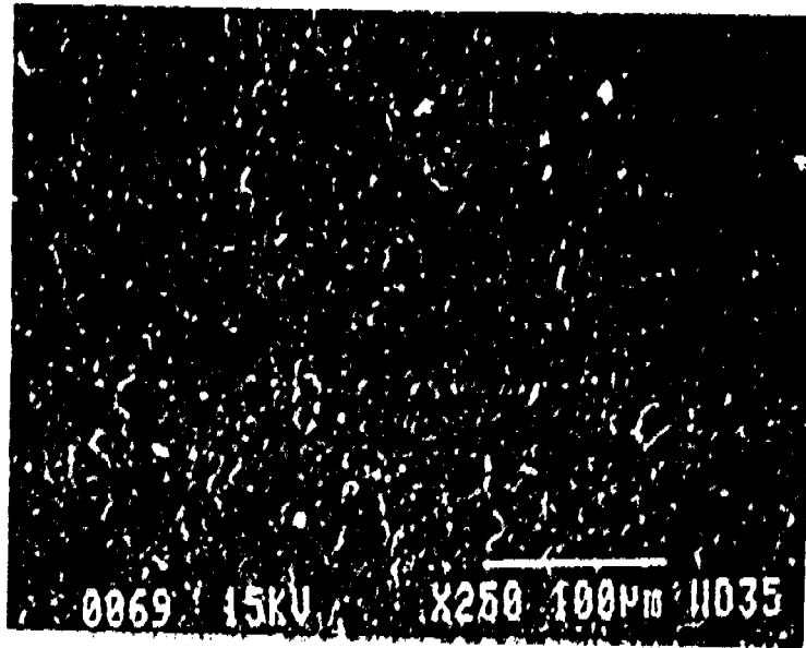
Figure 11. SEM photograph of the surface of a Clarity bracket ( as received ).
