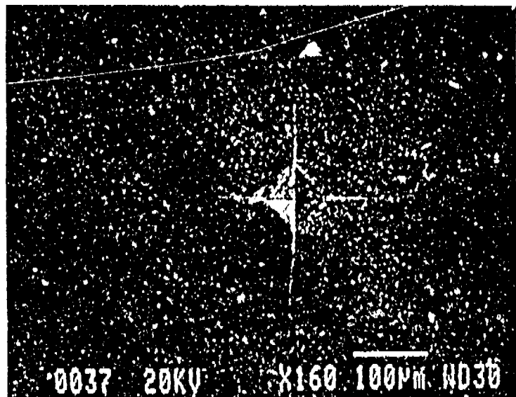
Figure 8. A 1 kg indentation on the polished base of a Contour bracket (low magnification).
