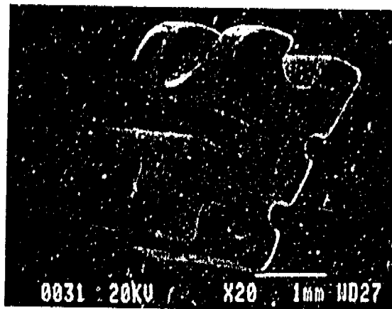
Figure 25. SEM photograph of an Allure NSB bracket: Archwire slot edge.
