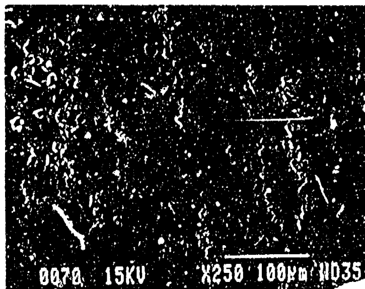
Figure 10. SEM photograph of the surface of an Allure NSB bracket ( as received ).
