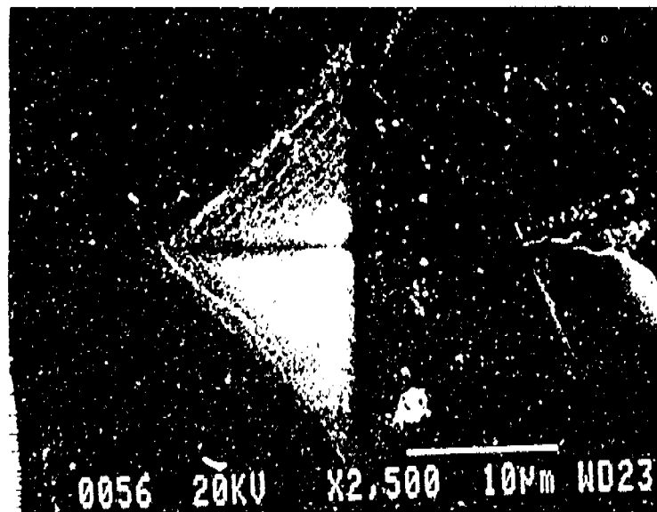
Figure 6. Scanning electron micrograph of a 1 kg indentation on the polished base of a Clarity bracket.
