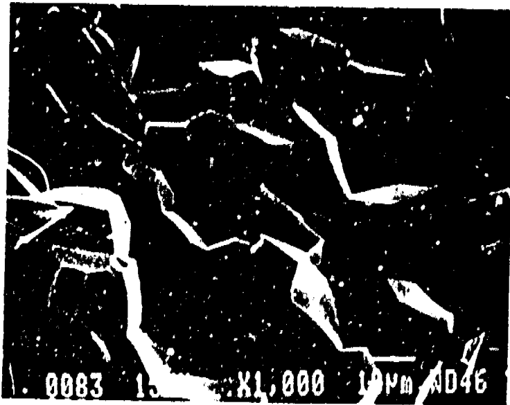
Figure 13. SEM photograph of the fracture surface of an Intrigue bracket.
