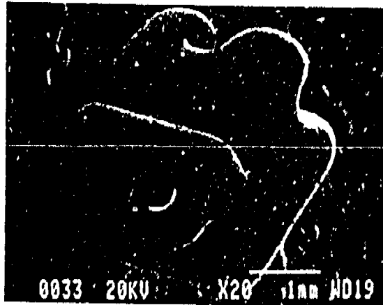
Figure 24. SEM photograph of an Allure NSB bracket: Archwire slot edge.
