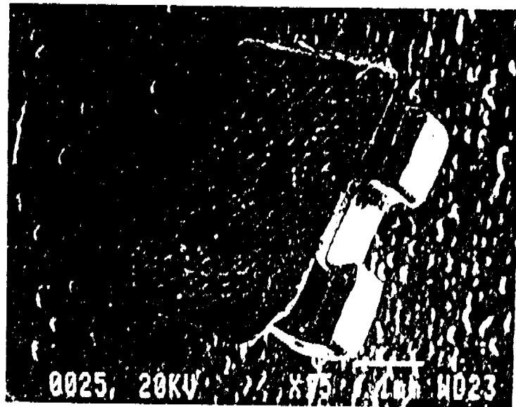
Figure 19. SEM photograph of the cast epoxy base of the MXi bracket.
