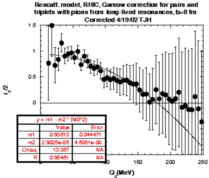
Figure 4.2: Simulation of effect of mis-applying the Coulomb correction to pions emitted from the decay of long-lived resonances. The upper plot shows the result with the Coulomb potential turned off, and the lower plot shows the result of applying the Coulomb correction to all pions, including those emitted from \eta , \eta' , K_S^0 and \Omega^- decays.
