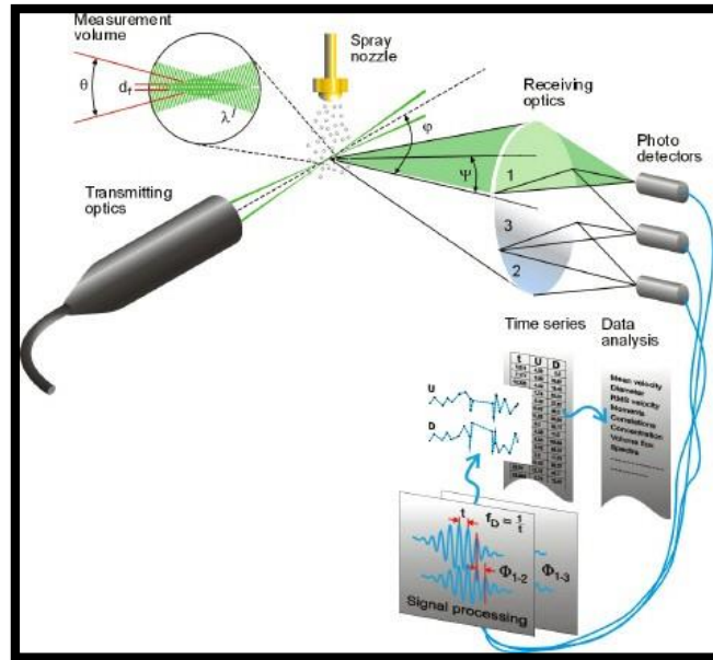
Figure 21: Overview of Particle Doppler Interferometry (Source: Dantec Dynamics)
