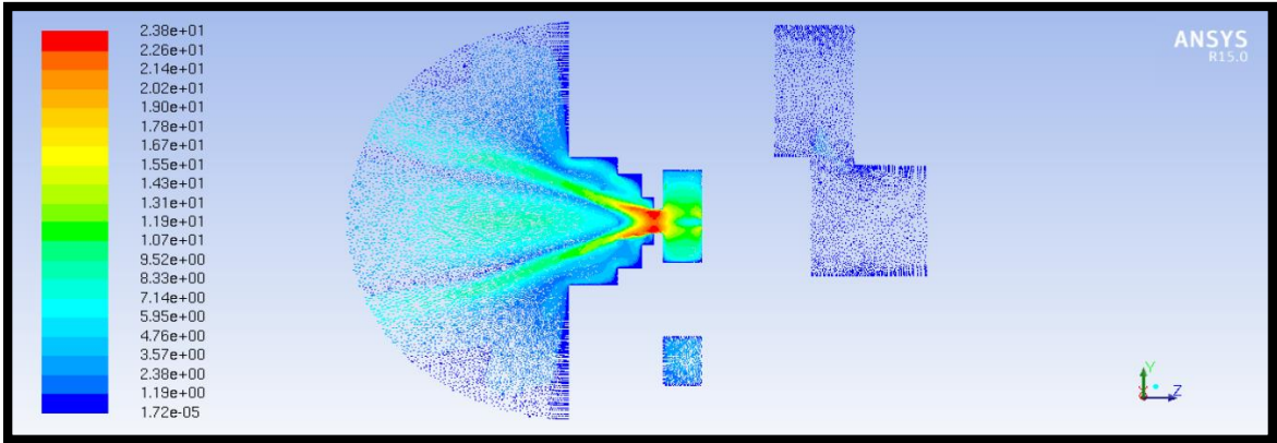
Figure 130: 40 psi, Macrospray Atomizer, Velocity Vectors
