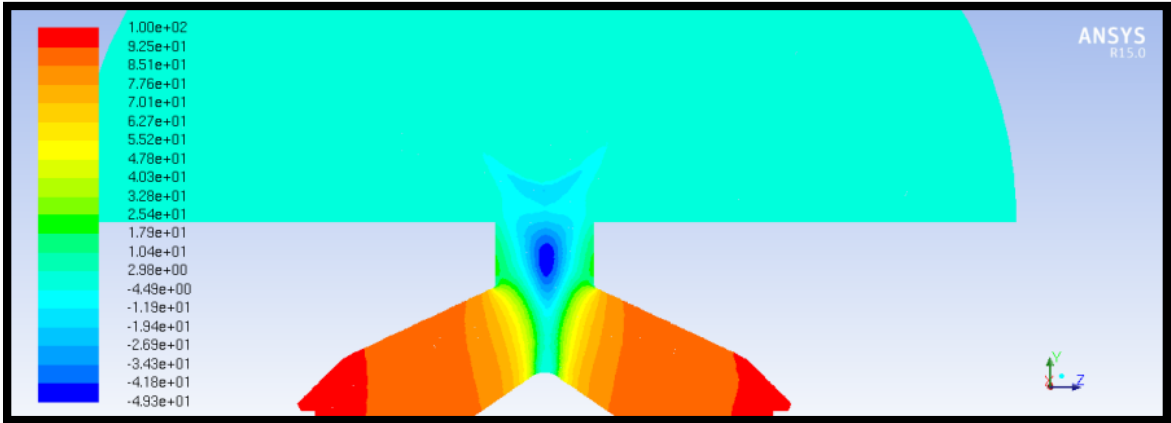
Figure 65: 100 psi, Conventional Atomizer, Pressure Contours, Orifice
