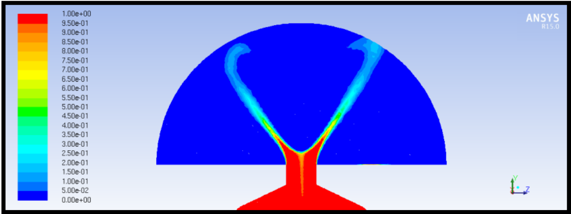
Figure 98: Volume Fraction, Conventional Atomizer, 3.8 million cells, Outlet
