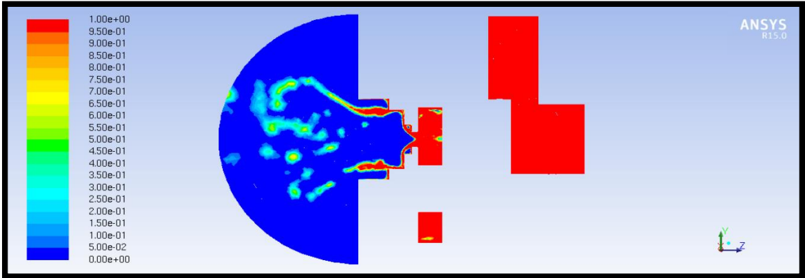
Figure 113: 20 psi, Macrospray Atomizer, Volume Fraction
