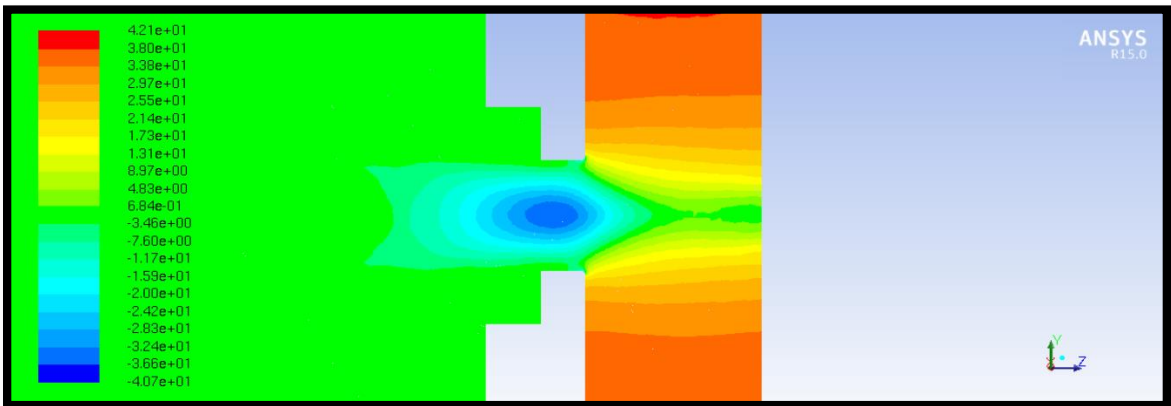
Figure 128: 40 psi, Macro Spray Atomizer, Pressure Contours, Orifice
