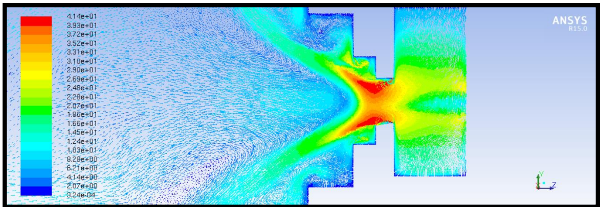
Figure 55: 145 psi, Macrospray Atomizer, Velocity Vectors, Air Core
