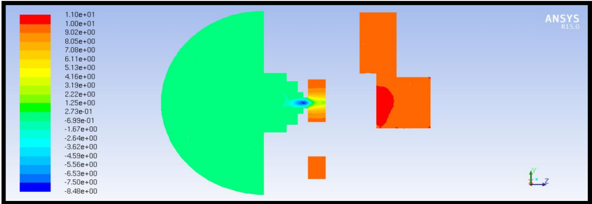
Figure 103: 10 psi, Macro-spray Atomizer, Pressure Contours
