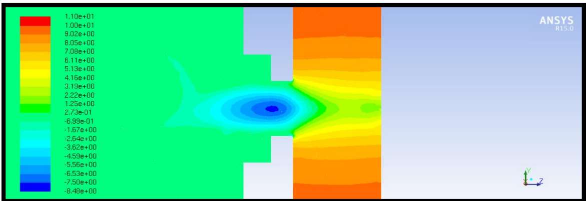
Figure 104: 10 psi, Macro-spray Atomizer, Pressure Contours, Orifice
