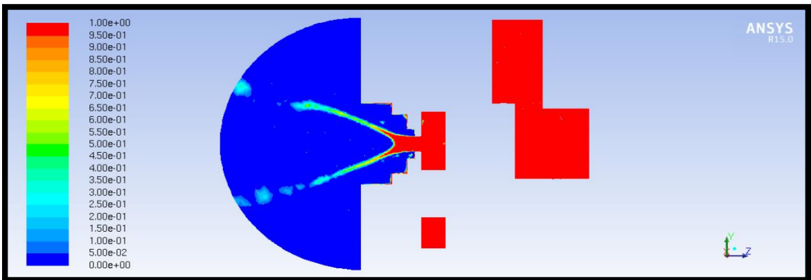
Figure 125: 40 psi, Macrospray Atomizer, Volume Fraction
