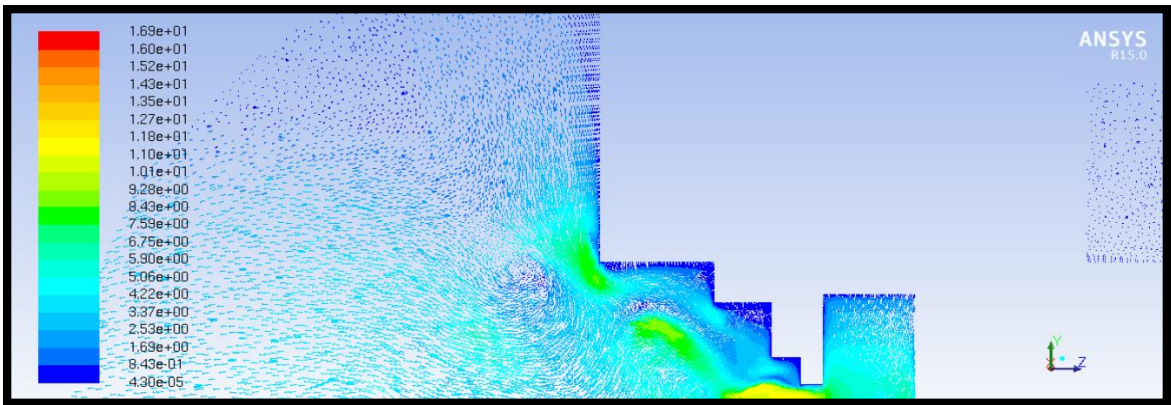
Figure 111: 10 psi, Macrospray Atomizer, Velocity Vectors, Jetstream Top
