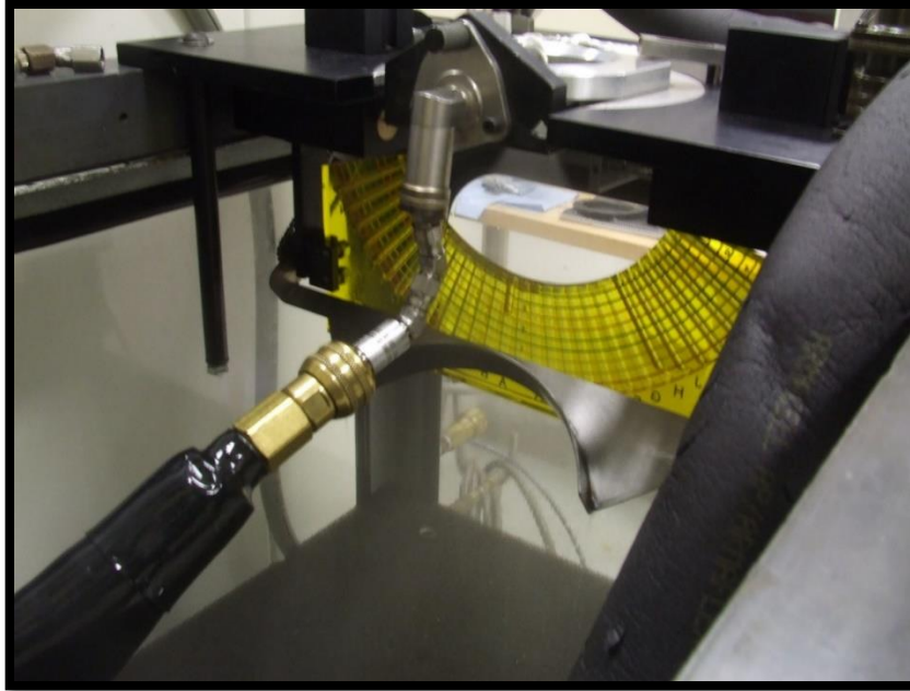
Figure 34: View of Test in Progress of Angle Device Setup, Conventional Atomizer (Source: Parker Hannifin Gas Turbine Fuel Systems Division)
