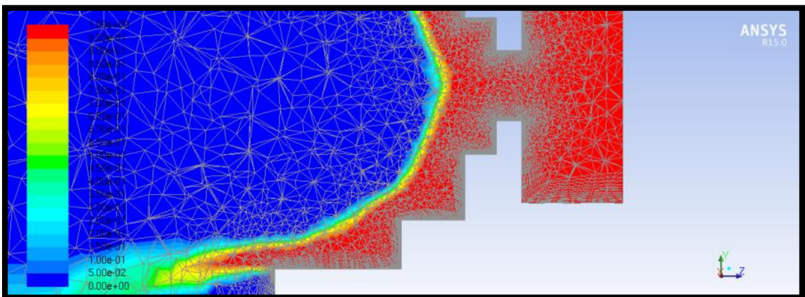
Figure 79: Meshed Volume Fraction, Macropray Atomizer, 1 million cells, Orifice
