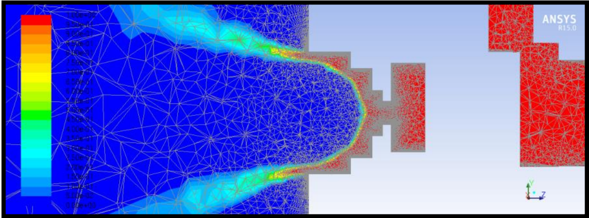
Figure 78: Meshed Volume Fraction, Macropray Atomizer, 1 million cells
