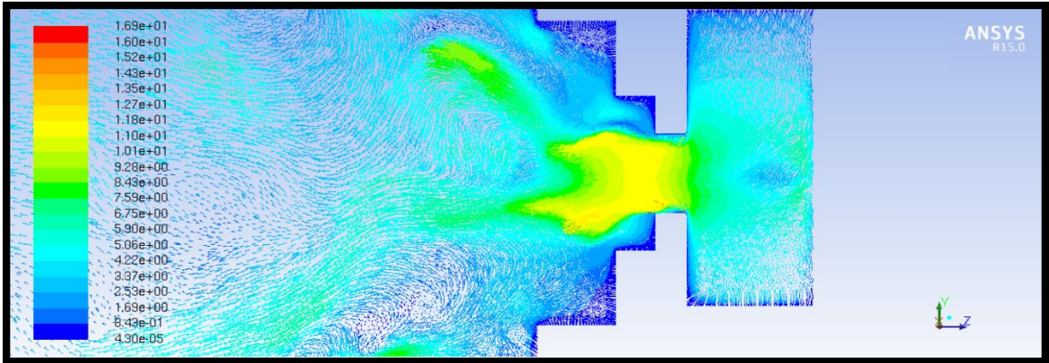
Figure 109: 10 psi, Macrospray Atomizer, Velocity Vectors, Air Core
