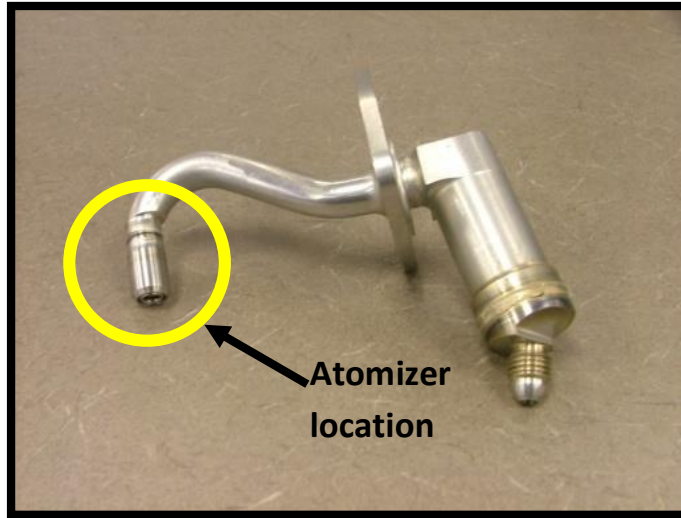
Figure 3: Atomizer Location Callout (Source: Parker Hannifin Gas Turbine Fuel Systems Division)
