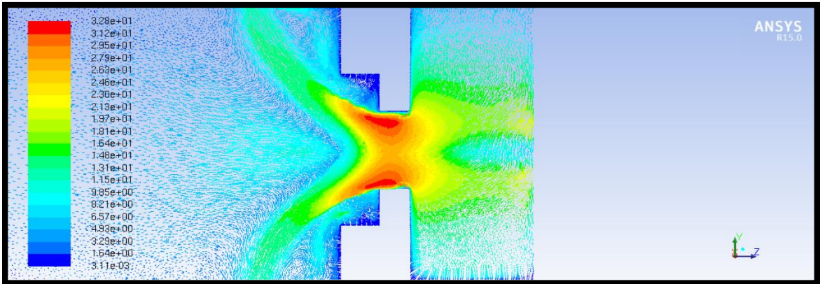
Figure 143: 80 psi, Macro Spray Atomizer, Velocity Vectors, Orifice
