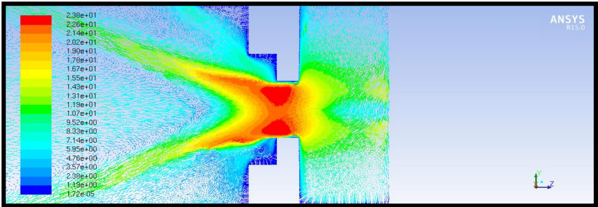
Figure 131: 40 psi, Macrospray Atomizer, Velocity Vectors, Orifice
