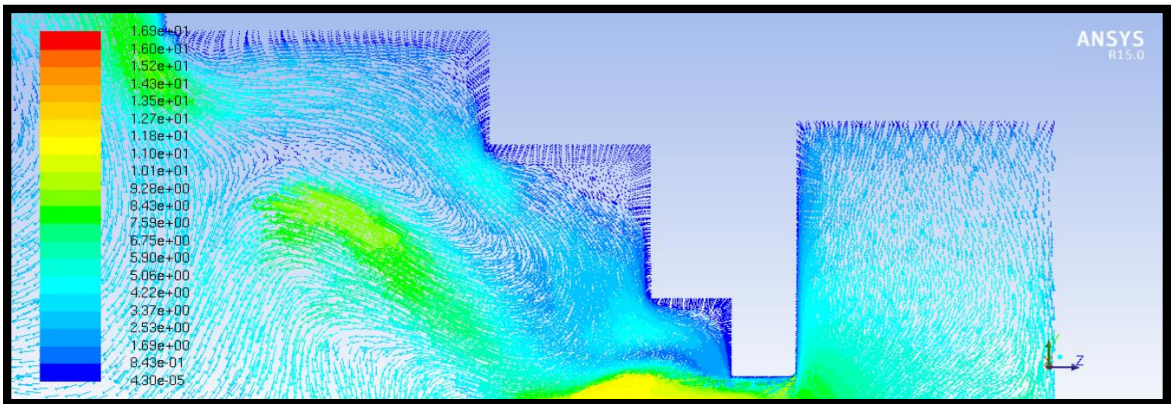
Figure 110: 10 psi, Macrospray Atomizer, Velocity Vectors, Recirculation Zones
