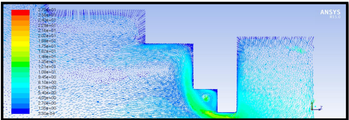
Figure 122: 20 psi, Macrospray Atomizer, Velocity Vectors, Recirculation Zones
