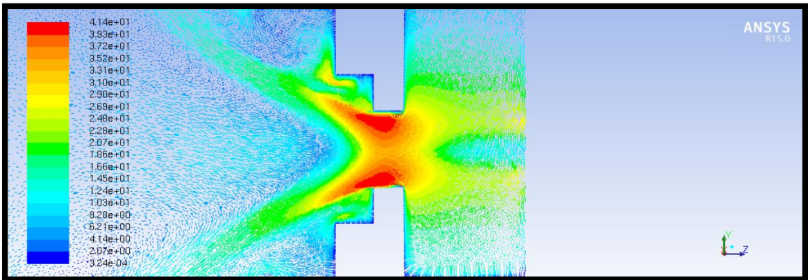
Figure 53: 145 psi, Macrospray Atomizer, Velocity Vectors, Orifice
