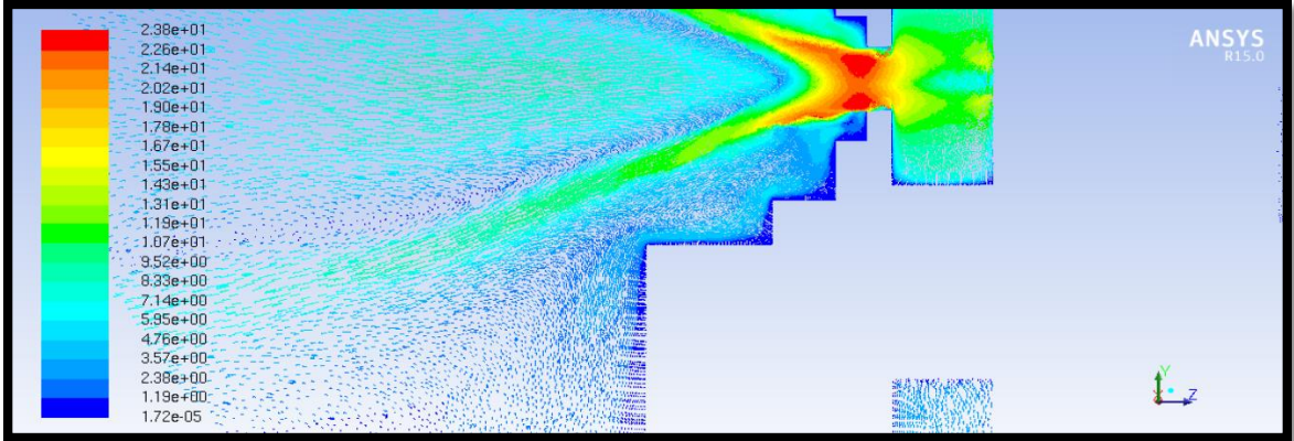
Figure 136: 40 psi, Macrospray Atomizer, Velocity Vectors, Jetstream Bottom
