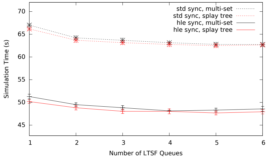
Figure 6.20: Multi-Set VS Splay Tree LTSF Queues for HLE using 6 Worker Threads
